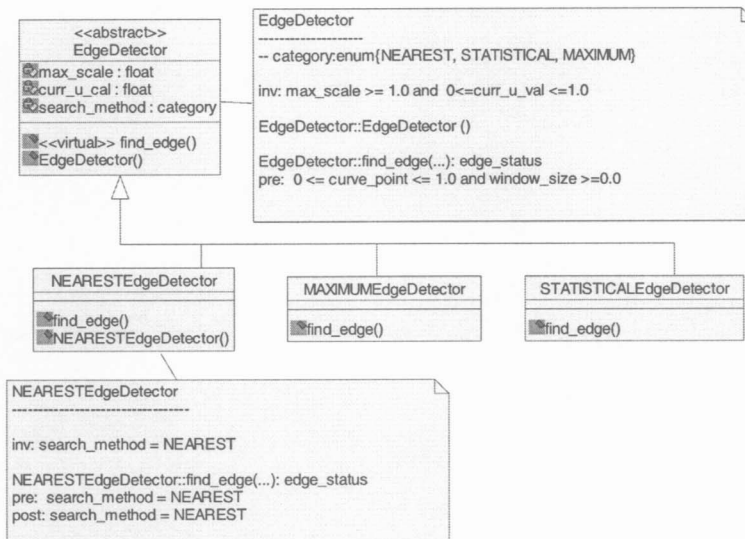
Figure 4. Refactoring: Replacing conditionals with polymorphism
