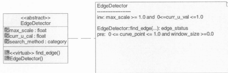
Figure 3. Class EdgeDetector: before refactoring
