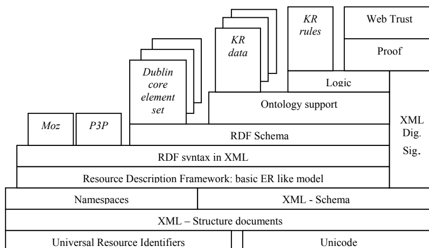
Figure 1: Semantic Web Language cake
