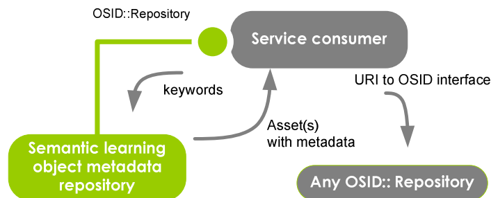
Figure 2. Non-semantic search on semantic repositories
