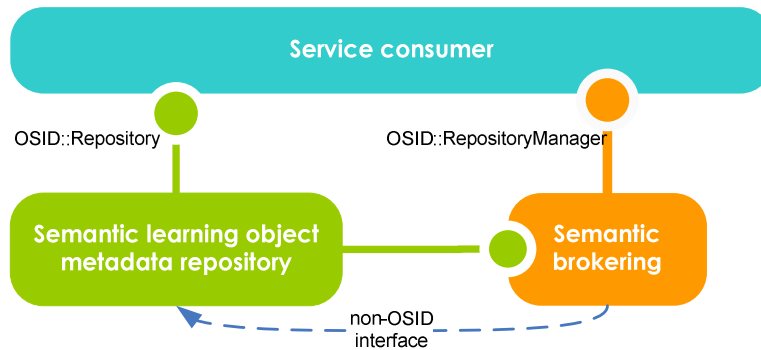
Figure 1. Approximation to support semantic search using OSID.
