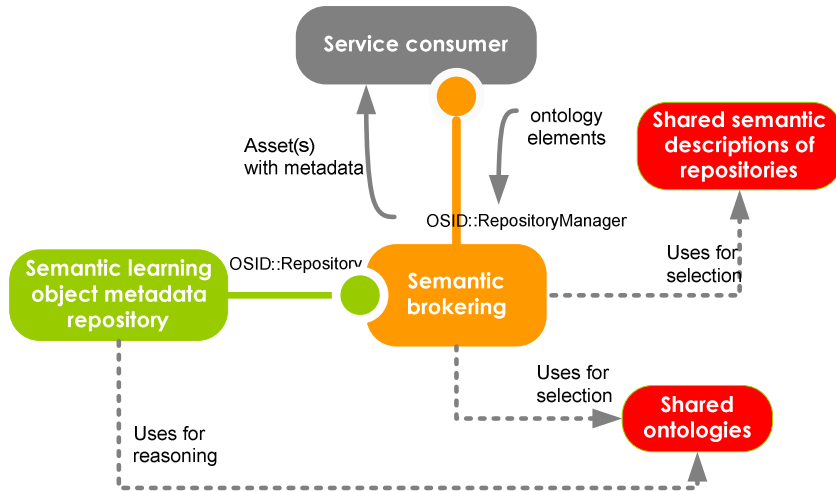
Figure 4. Brokered semantic query
